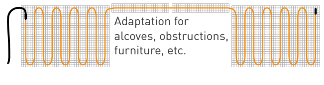
Adjustment directly after the PTC thermistor
